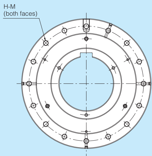
Chamfer of the bore end faces
