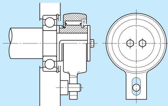
Typical Installation 2
