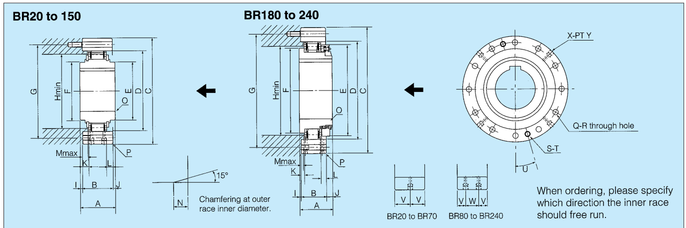
Dimension (Open Type)
