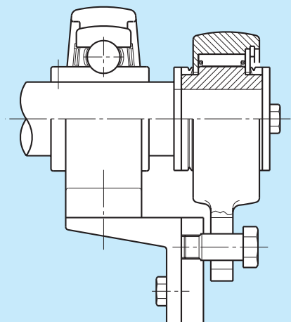
Typical Installation 1
