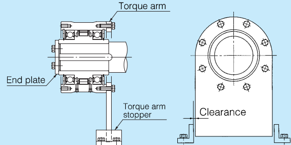
Installation example 1:
